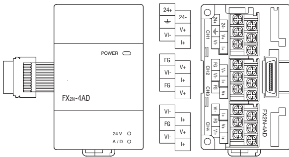
FX2N-4AD
