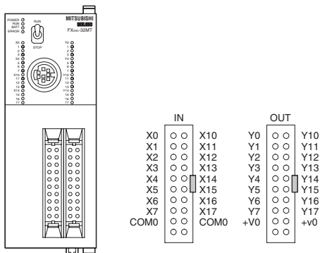
FX2NC-32MT-DSS
